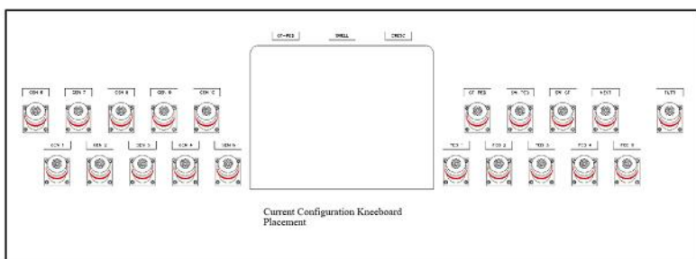
Kneeboard Layout
